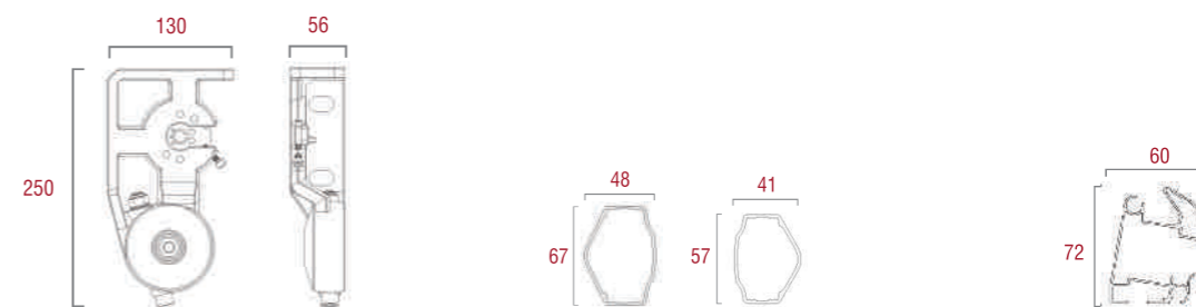
supporto universale universal fixing bracket
